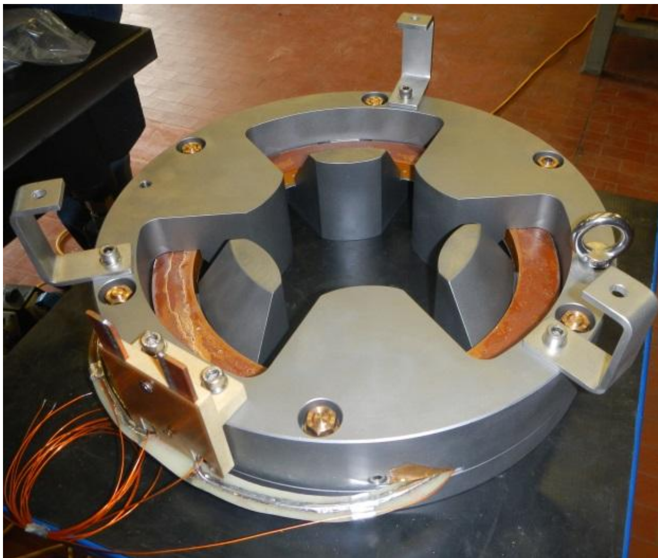
Figure 2: A module of the RCSM assembled and ready to be tested
