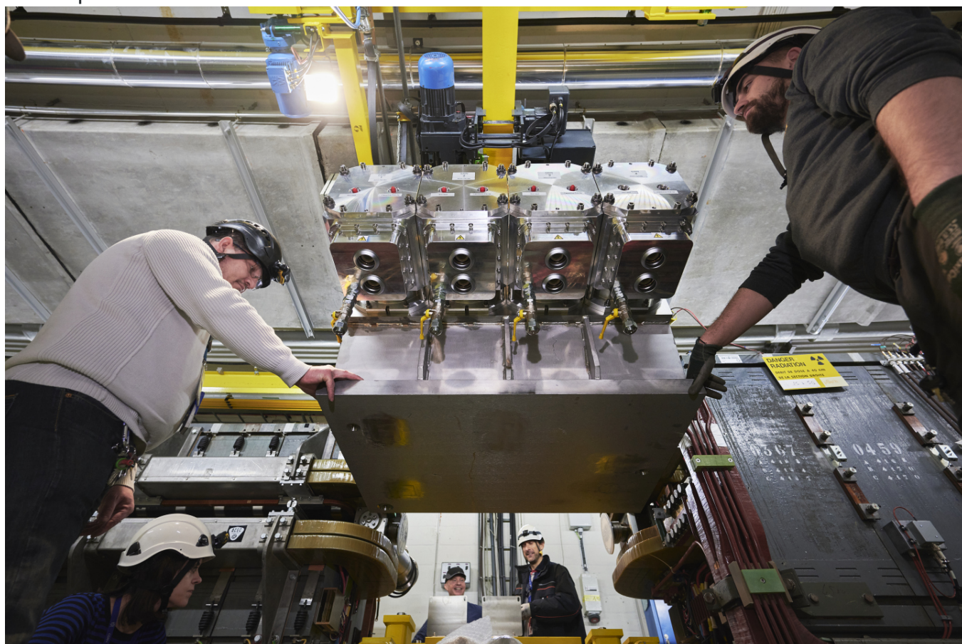
The new kicker for the PS being installed in the accelerator (Image: Julien Ordan/CERN)
