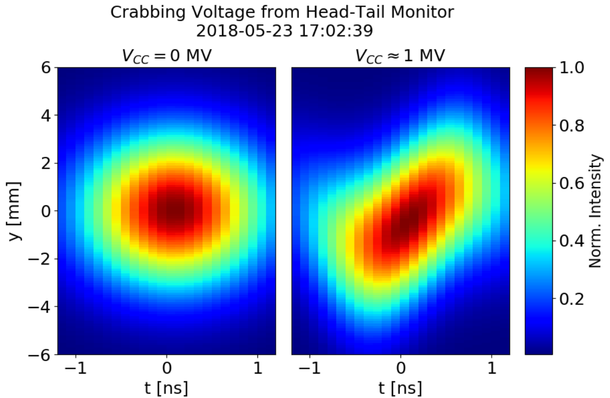
Figure 3: Images a bunch in the CERN SPS for 2 different voltage settings in the Crab Cavities. Left without voltage and deflection. Right with 1MV voltage and deflection.
