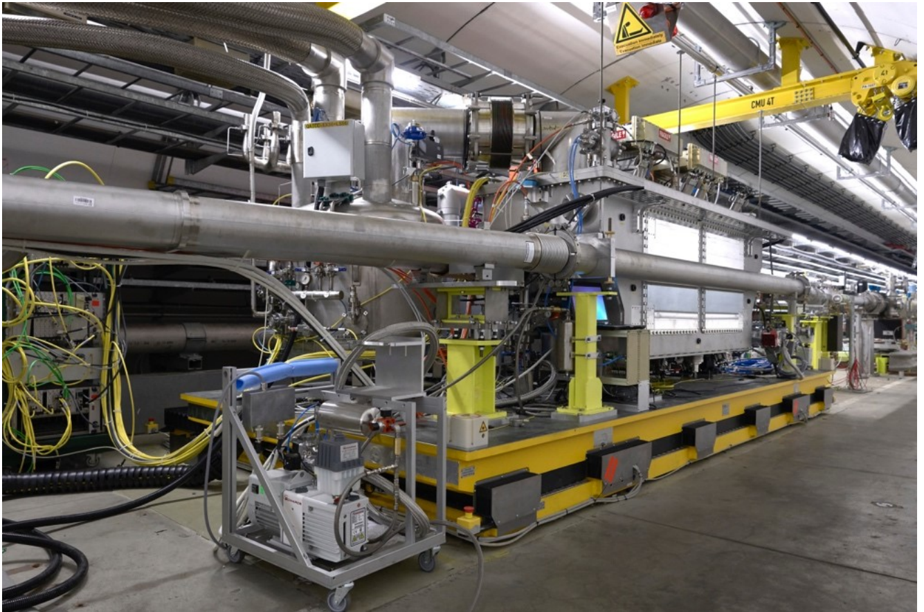
Figure 2: The Crab Cavity Cryostat installed on a movable table in the CERN SPS.
